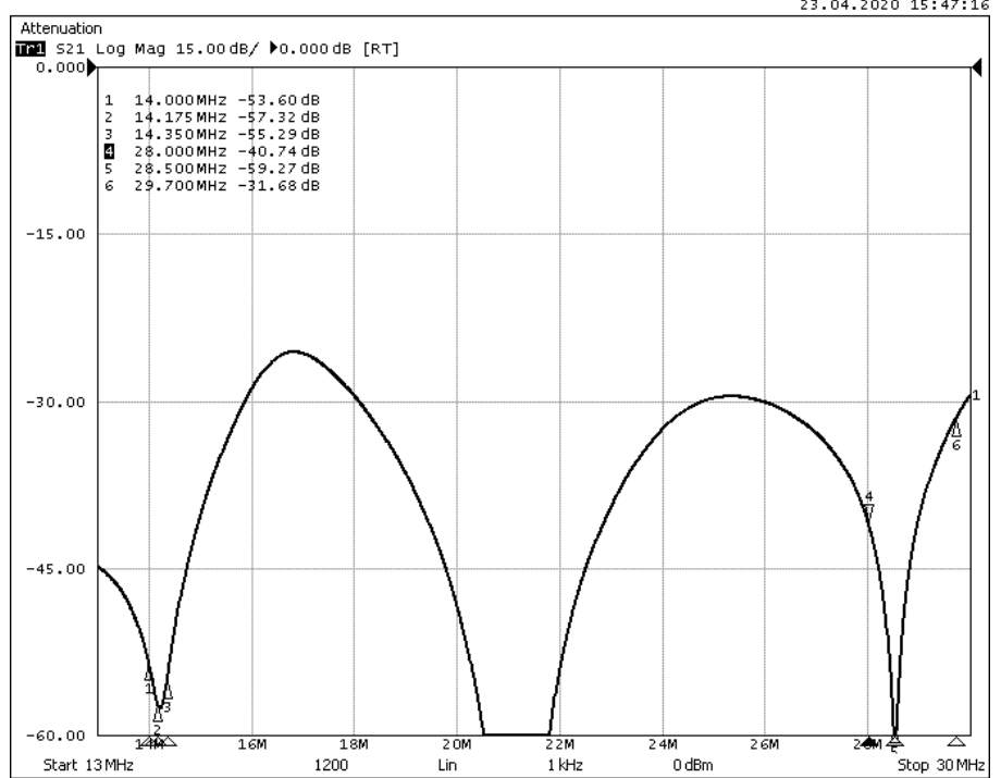
Isolation: 14MHz port to 28MHz port
