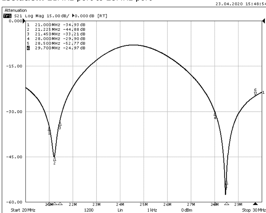
Isolation: 21MHz port to 28MHz port
