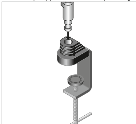
Abb. 1: Mounting the fastening element.
