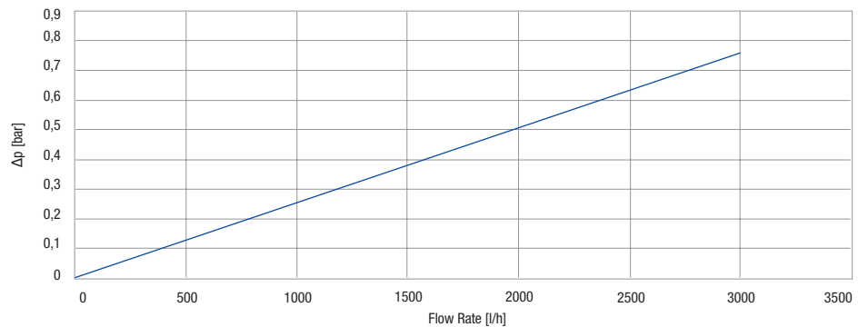
Tests carried on 10" elements type LA Ag 10 BIG SX . Testing mode: 20°C, 3 BAR
