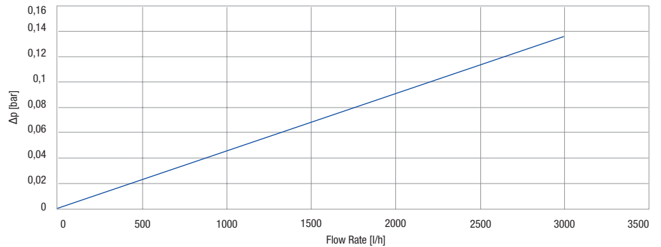
Tests carried on 10" elements type LA 10 BIG SX . Testing mode: 20°C, 3 BAR
